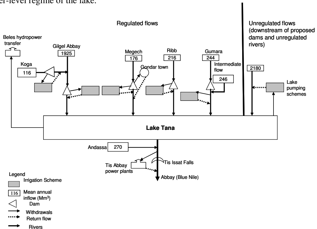
Figure 3: Schematic of existing and planned water demand in the Lake Tana catchment as simulated in WEAP, showing the mean annual flow upstream of the proposed irrigation dams as well as unregulated flows into the lake.
